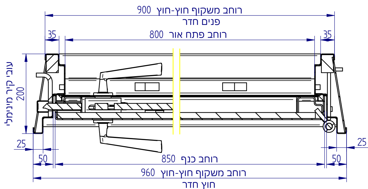
SECTION B-B
